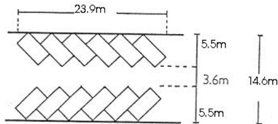
45° PARKING
