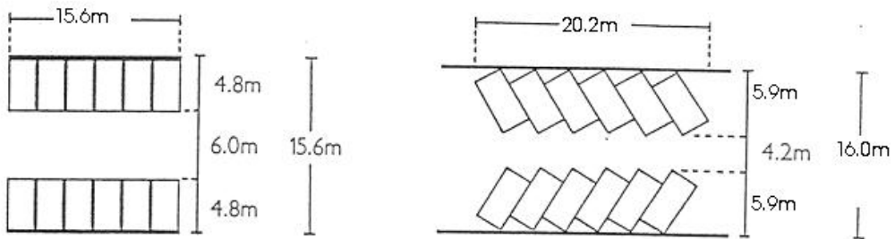
90° PARKING
