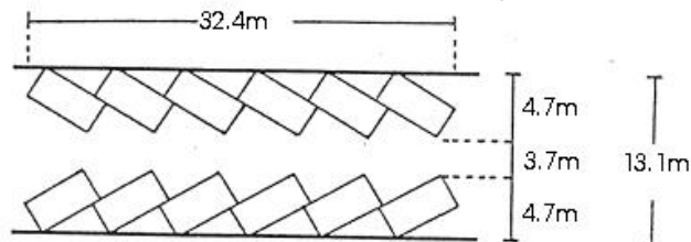
30° PARKING
